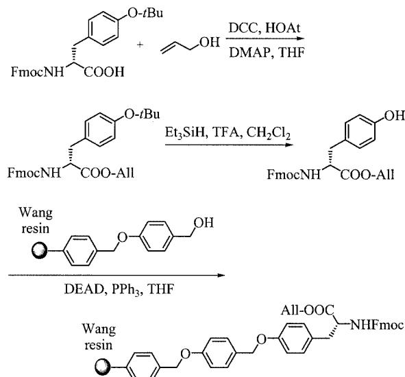
Scheme 2. Modification of Wang resin
