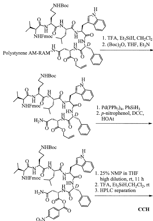
Scheme 6. Synthesis of the central cyclic hexapeptide CCH by non direct in situ cyclization in solution
