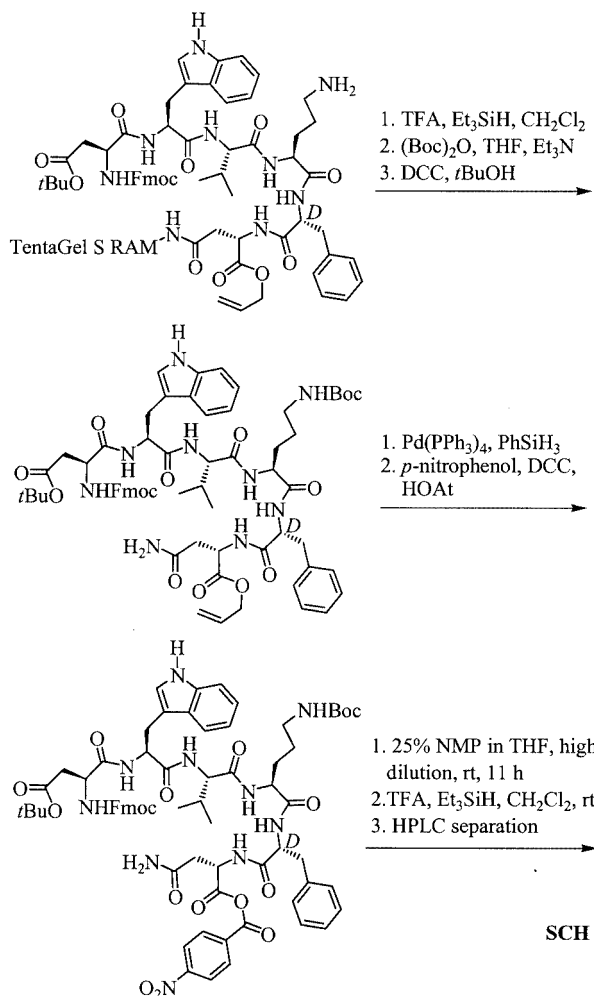
Scheme 5. Synthesis of the southern cyclic hexapeptide SCH by indirect in situ cyclization in solution
