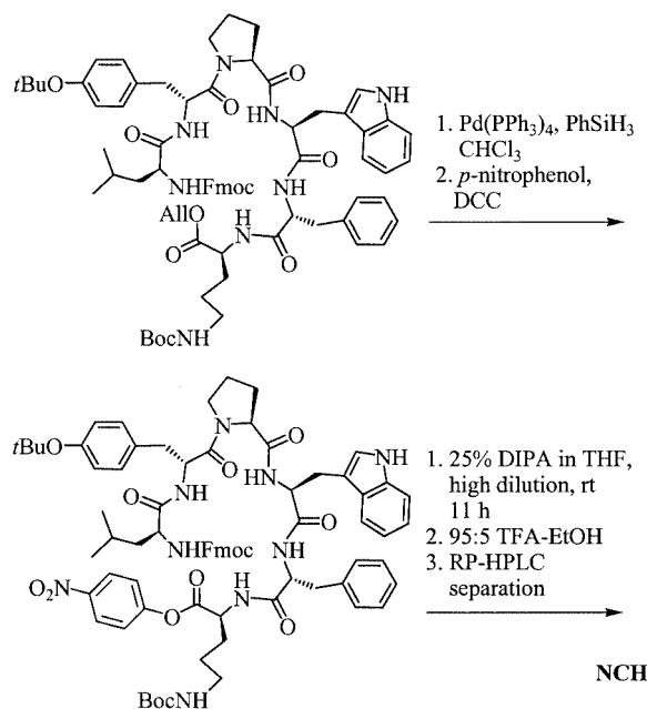
Scheme 4. Synthesis of the northern cyclic hexapeptide NCH by indirect in situ cyclization in solution
