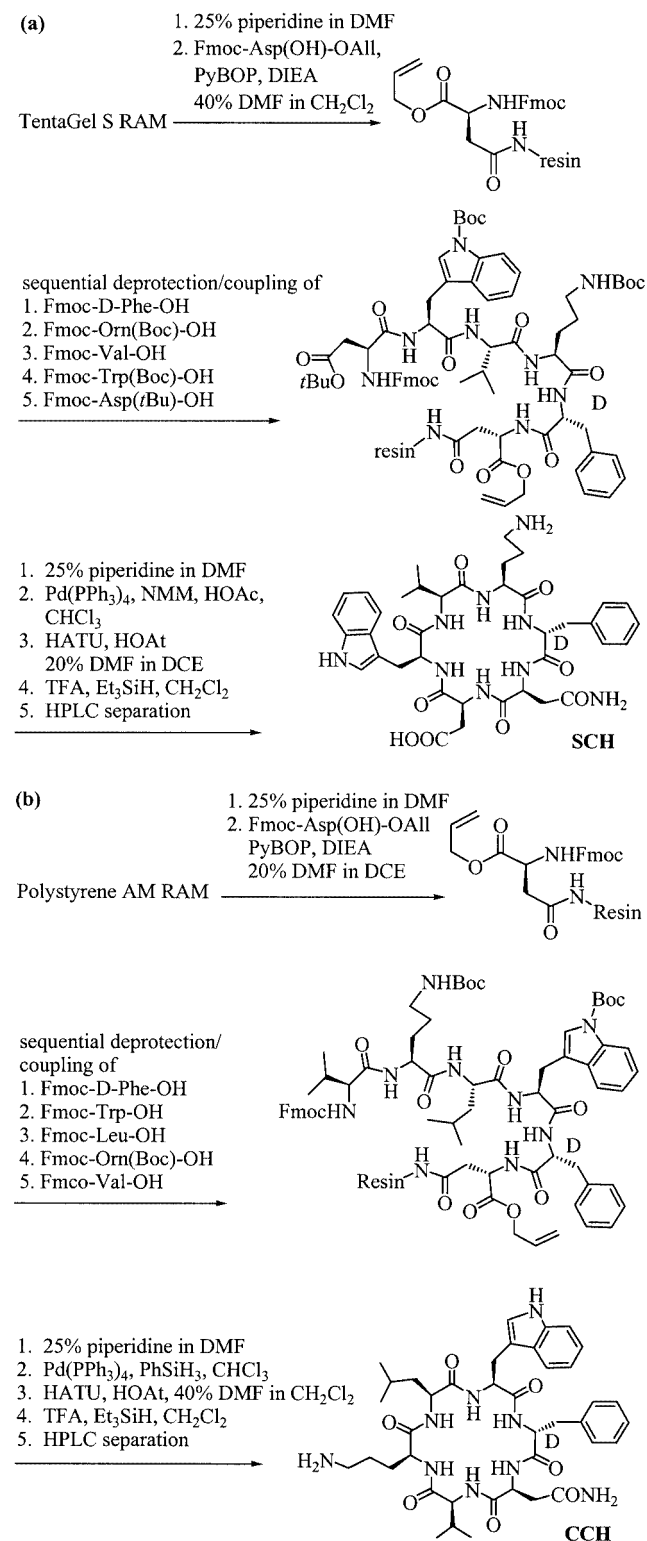
Scheme 1. Fmoc-based solid-phase synthesis of: (a) southern cyclic hexapeptide SCH (resin = TentaGel S RAM) and (b) central cyclic hexapeptide CCH (resin = polystyrene AM RAM)
