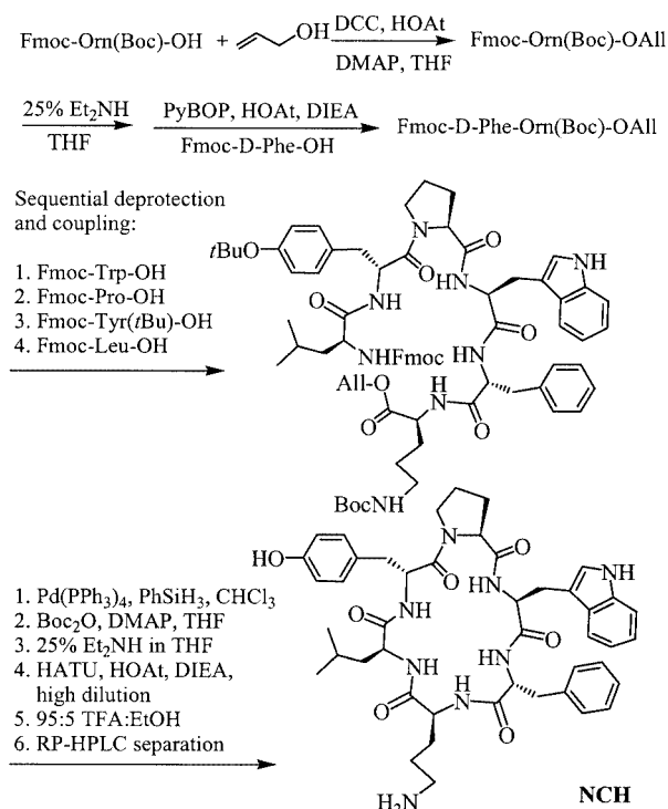
Scheme 3. Assembly of the linear hexapeptide precursor and its conversion into the northern cyclic hexapeptide NCH by the direct cyclization method
