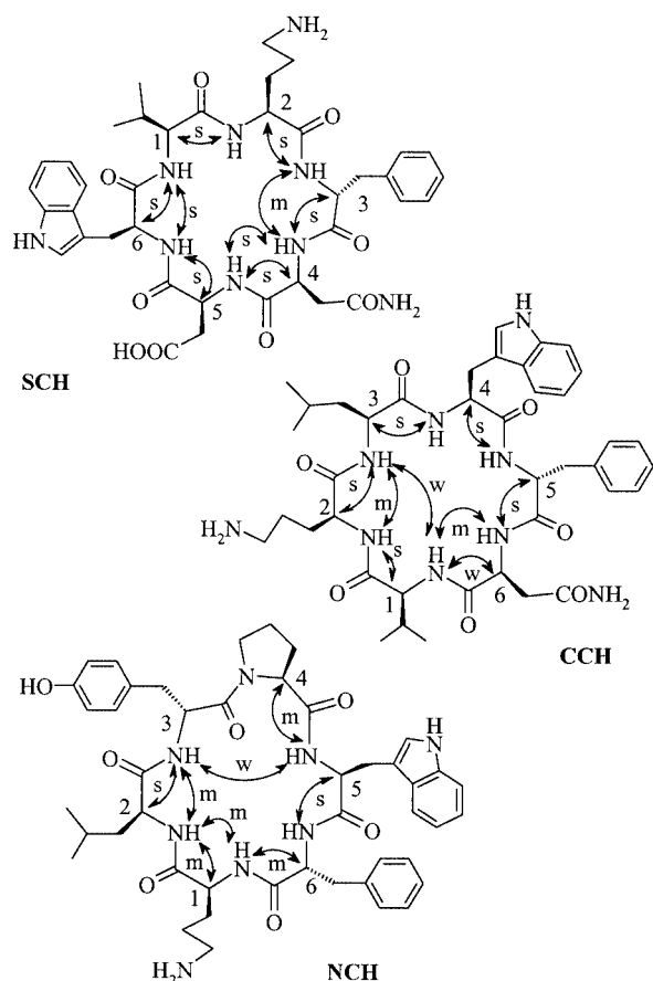
Figure 3. Important NOEs of the southern cyclic hexapeptide (SCH), central cyclic hexapeptide (CCH), and northern cyclic hexapeptide (NCH) (s: strong; m: medium; w: weak)
