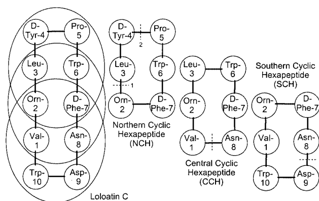
Figure 2. 'Sliding window' analysis of loloatin C to provide three cyclic hexapeptides, and retrosynthetic analysis of the cyclic hexapeptides
