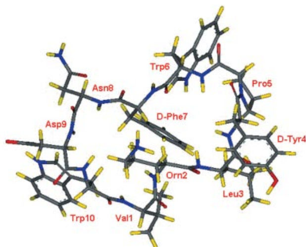
Figure 1. Structure of loloatin C and solution-state conformation in trifluoroethanol/water (70:30) as established by NMR spectroscopy and molecular simulation (ref. [4] )
